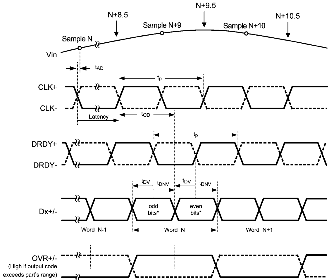
Output Timing
