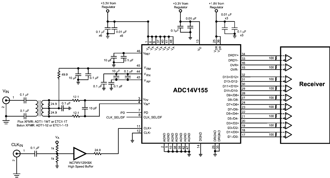
FIGURE 4. Application Circuit using Transformer Drive Circuit
